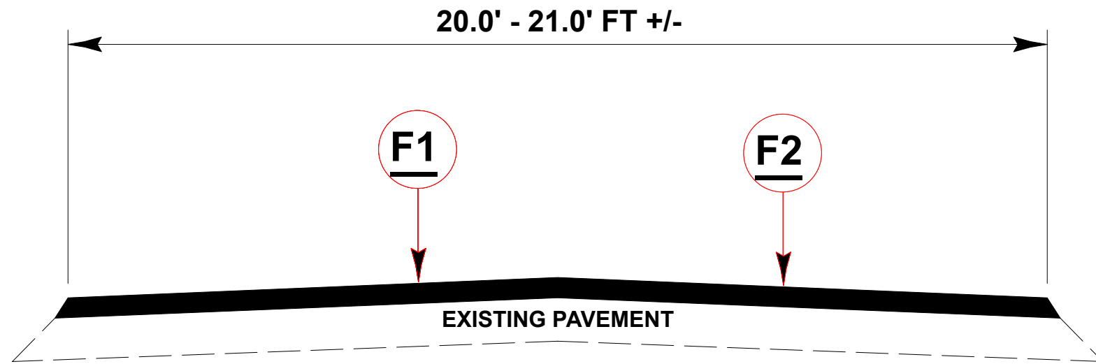
TYPICAL SECTION # 2 MAP(S) # 3 - 4
