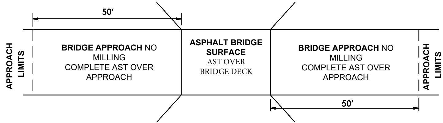
DETAIL FOR MAP # 3 & 4 / STRUCTURE # 0133, # 0159, & # 0164
